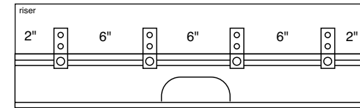
ProTop Contractor (Portable) (22" long)
